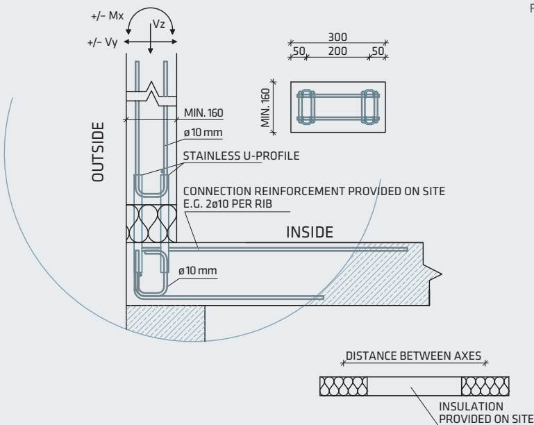
Fig. 23: Use of type XII-AT 2 for a parapet connection
