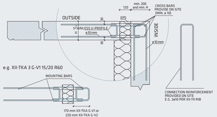
Fig. 15: Balcony connection – wall below with XII-TKA G-V1 or V2
