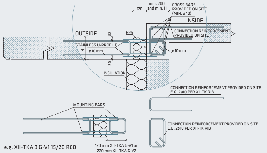
Fig. 19: Balcony with level change downwards with XII-TKA G-V1 or V2
