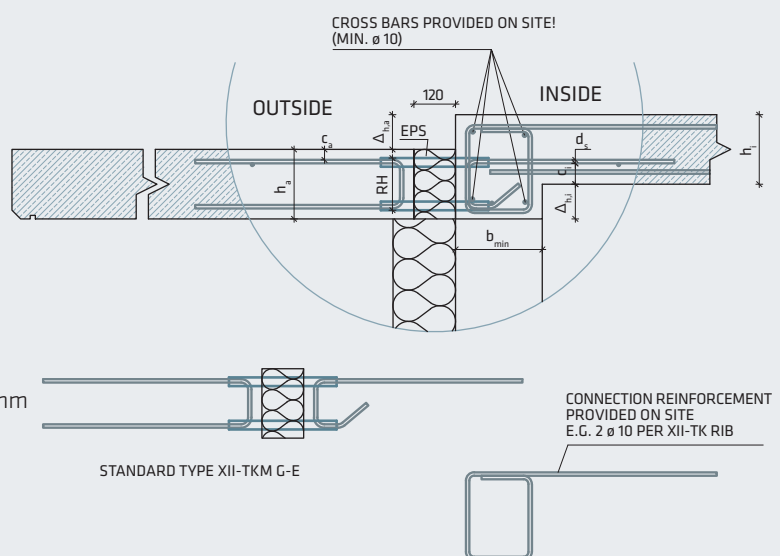
Fig. 5: Balcony with small level change downwards with XII-TKM G-E rib
