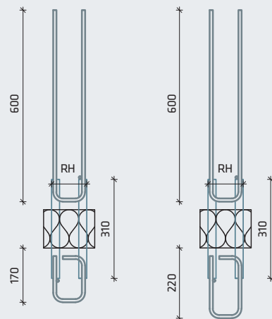
Fig. 24: XII-AT 2 G-V1 and V2
