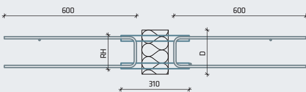
Fig. 2: Types of ribs of the type series XII-TKM
