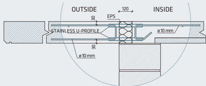
Fig. 4: Cantilevered balcony slab with XII-TKM G-E rib
