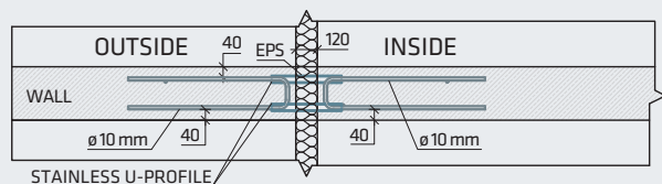
Fig. 21: Wall connection with XII-TKM G-G rib and XII-TKA G-V1 rib (elevation and sections)
