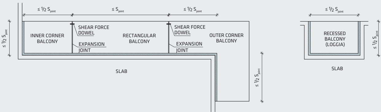
Fig. 29: Spacing of expansion joints
