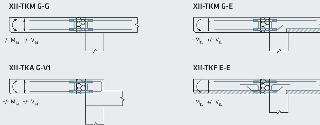
Fig. 25: Thermokorb load-bearing behaviour – transferable forces
