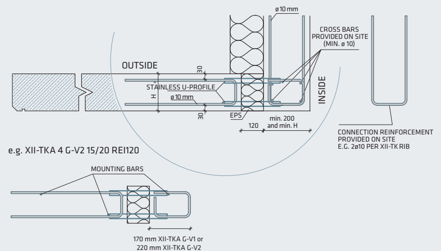
Fig. 16: Balcony connection – wall above with XII-TKA G-V1 or V2
