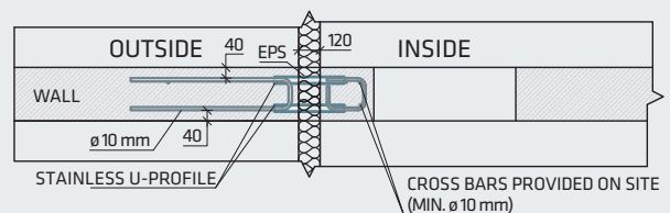
Fig. 21: Wall connection with XII-TKM G-G rib and XII-TKA G-V1 rib (elevation and sections)
