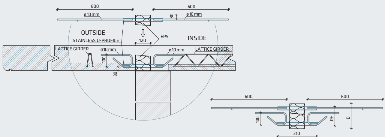
Fig. 12: Cantilevered balcony slab with split XII-TKF E-E rib
