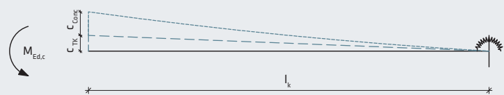
Fig. 26: Camber of a balcony slab
