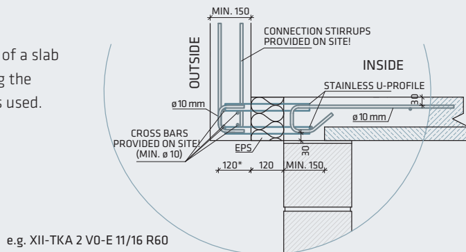
Fig. 20: Parapet in front of slab with XII-TKA V0-E rib
