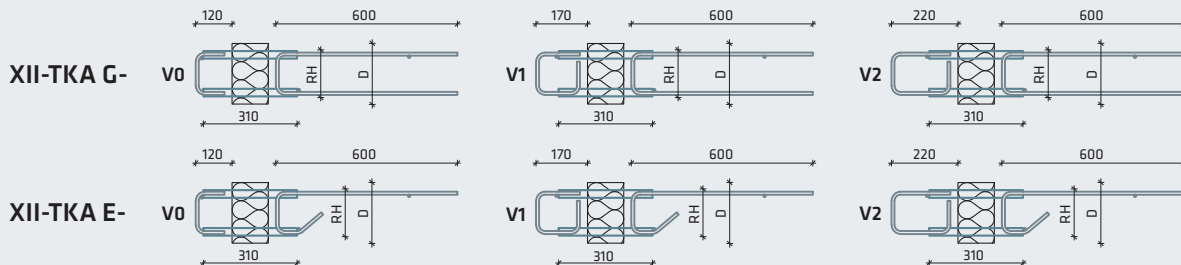
Fig. 14: Rib types of the type series XII-TKA
