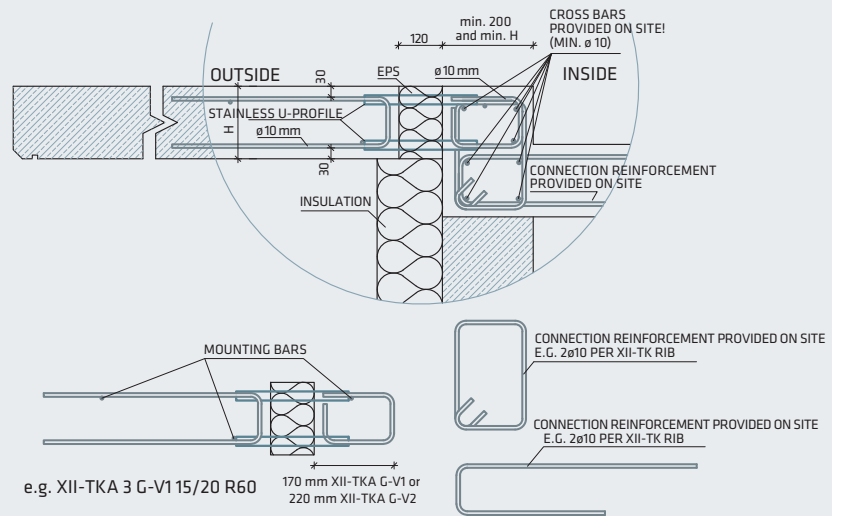
Fig. 18: Balcony with level change upwards with XII-TKA G-V1 or V2
