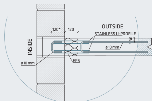
Fig. 17: Recessed balcony XII-TKA G-V0 Rib
