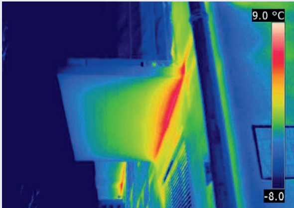
Fig. 27: Uninsulated connection area
