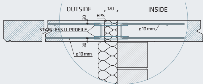
Fig. 3: Cantilevered balcony slab with XII-TKM G-G rib
