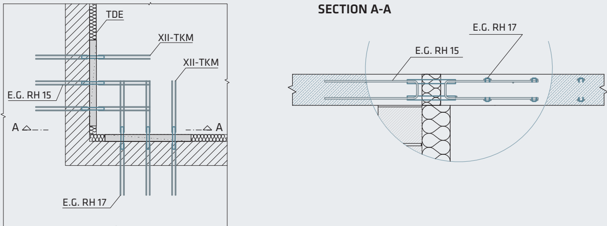
Fig. 30: Corner design with the Thermokorb® XII-TK
