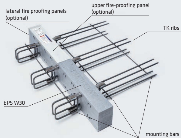
Fig. 13: XII-TKA G-V2 example with/without fire-proofing panels
