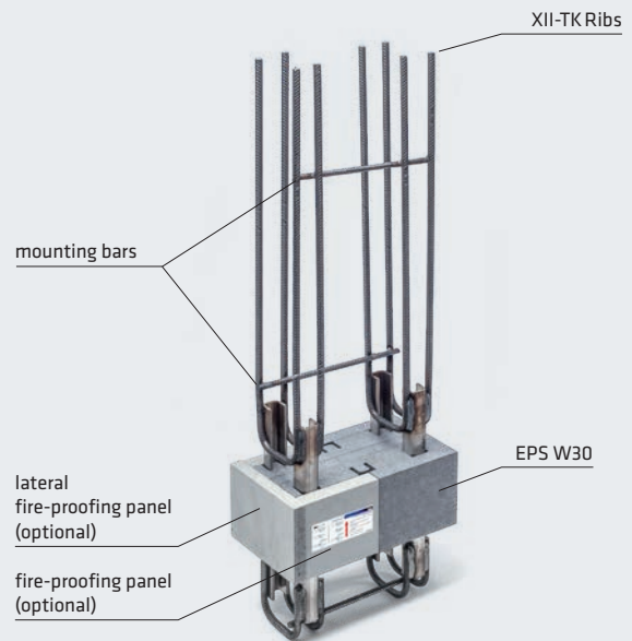
Fig. 22: XII-AT 2 example with/without fire-proofing panels
